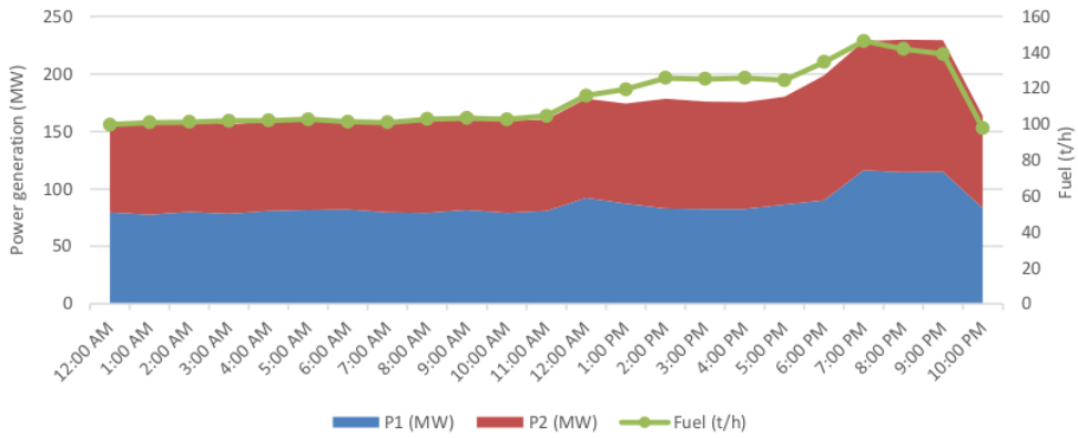
Figure 1. Current dispatch at the Jenepono Thermal Power Plant
