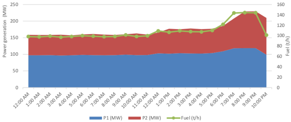
Figure 2. Economic dispatch results for the Jenepono Thermal Power Plant
