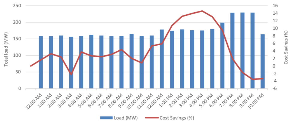
Figure 4. Cost savings for each total load
